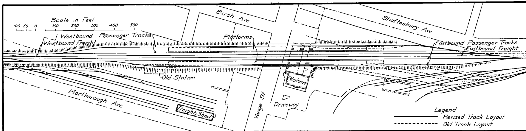
Track Arrangement in Vicinity of New North Toronto Station..
