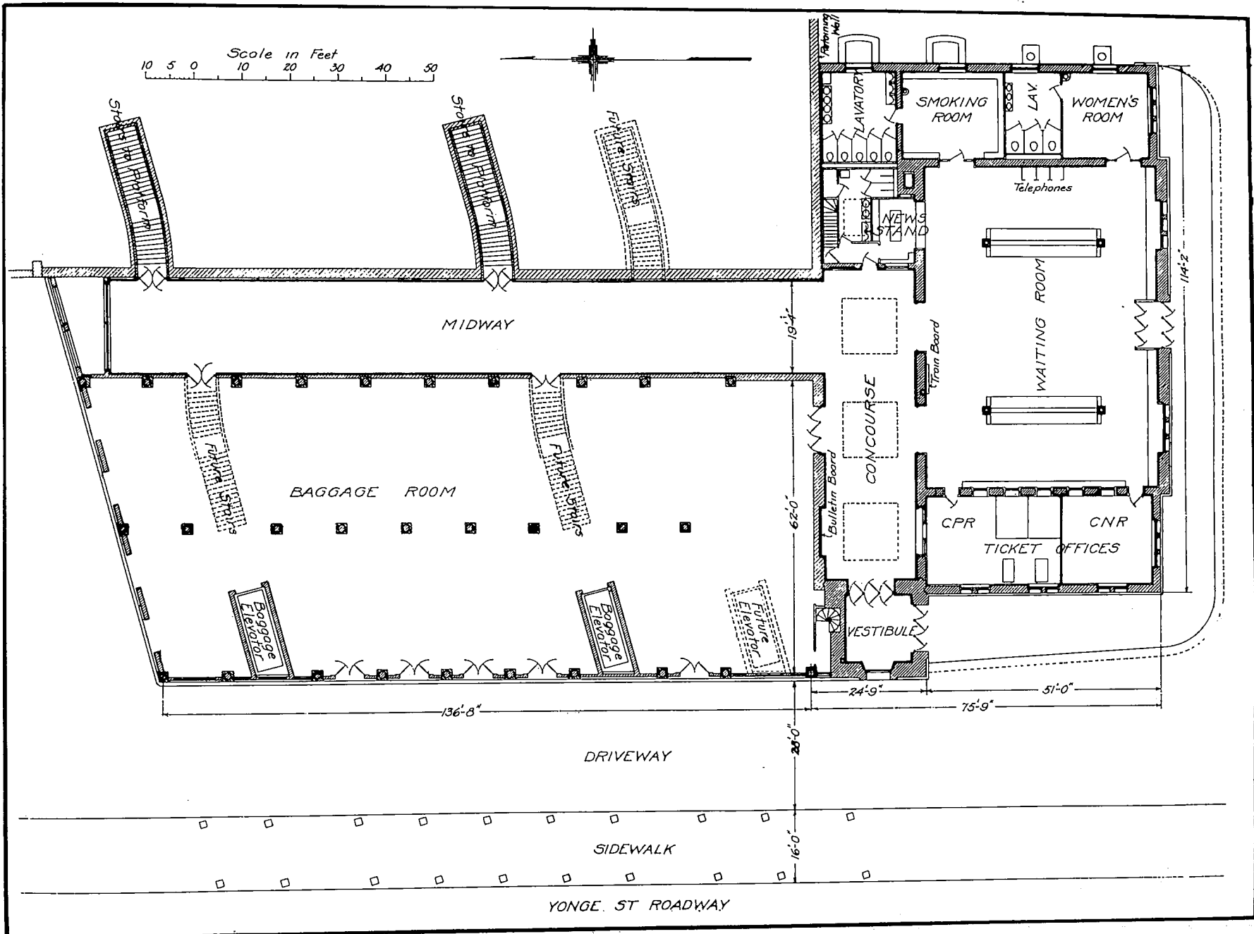
Ground Floor Plan of New North Toronto Station.
